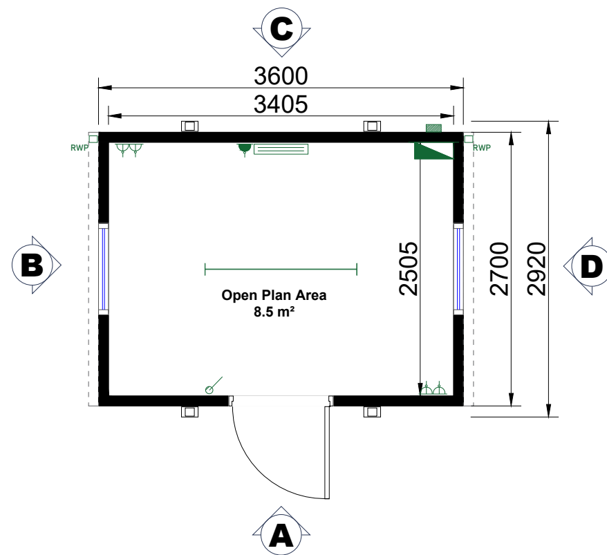
12' x 9' (3.6m x 2.7m) Portable Cabin
