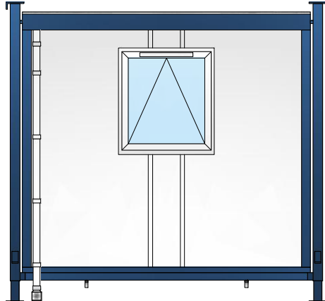
Elevation D
