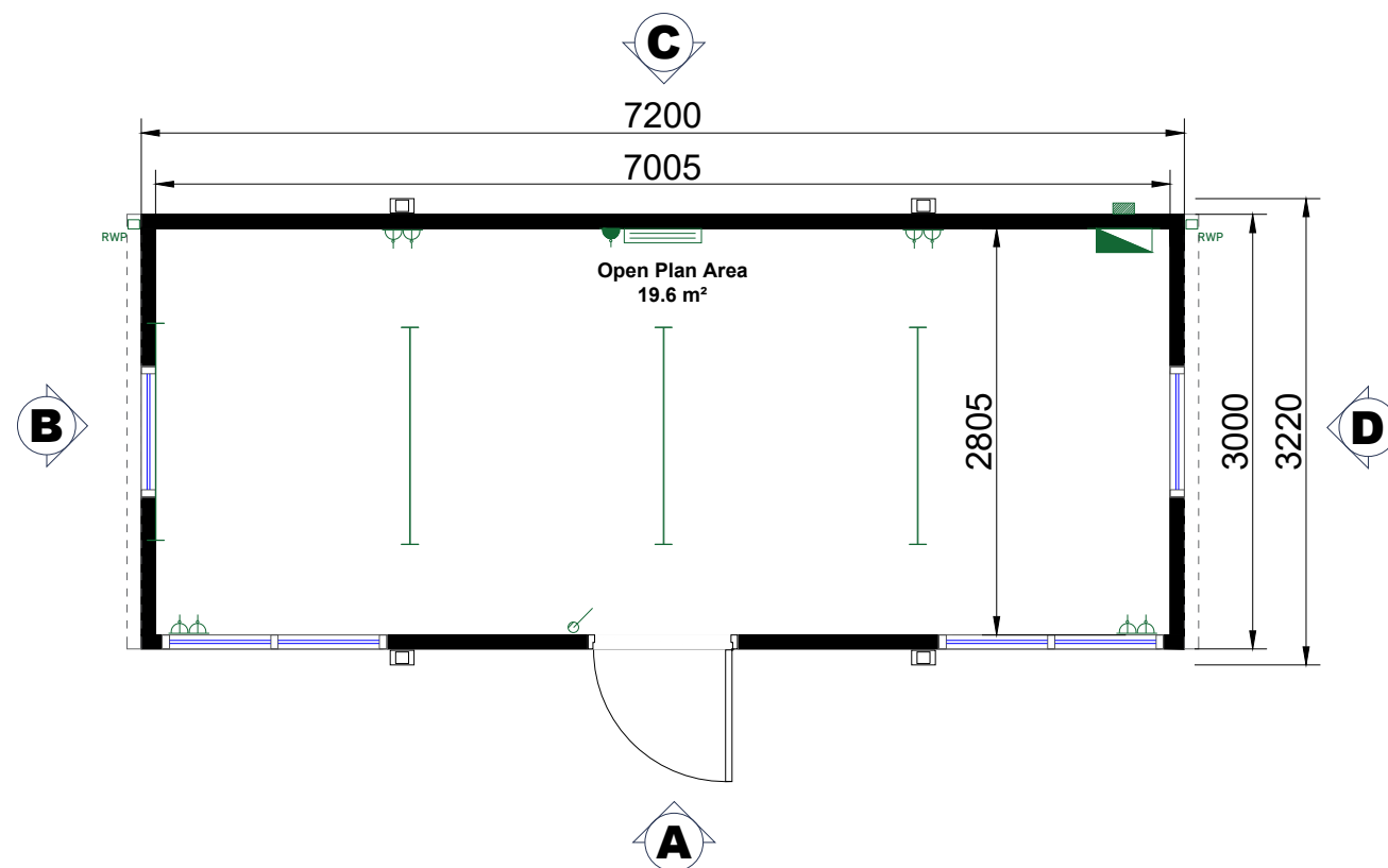
24' x 10' (7.2m x 3.0m) Portable Cabin
